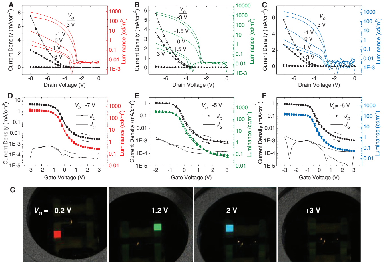
Fig. 2. CN-VOLET device operation. (A to C) Output and (D to F) transfer J - L - V curves of the (A and D) red, (B and E) green, and (C and F) blue CN-VOLETs. (G) Images of the corresponding color CN-VOLET pixels (1 mm by 1 mm) below the
